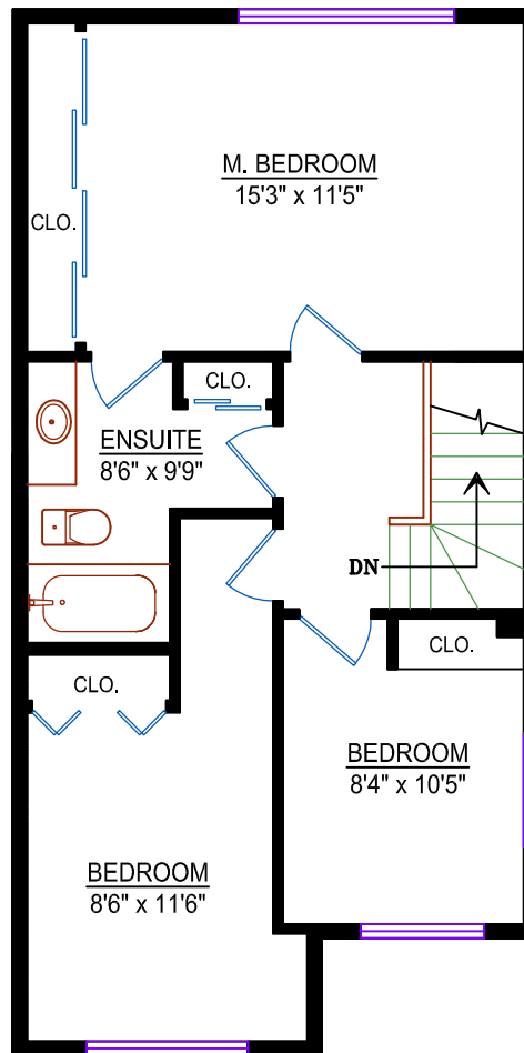
UPPER LEVEL Area: 624 sq. ft.
